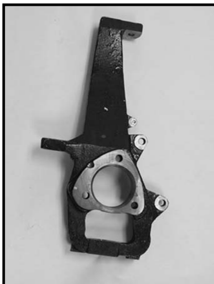
Part # 34100-01 / Qty. 1 Driver side knuckle
